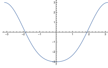
Figure 5.8: Fig of -(\sin^2 \phi + 3 \cos \phi)
